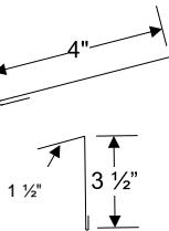
EAVE TRIM
