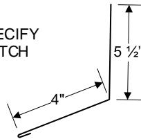
ENDWALL FLASHING
