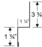
SIDEWALL FLASHING
