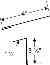
EAVE TRIM
