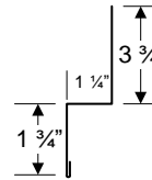
SIDEWALL FLASHING
